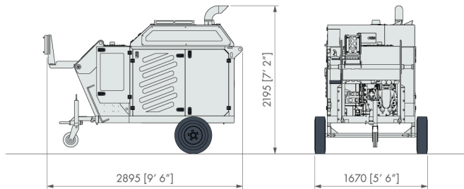
DIESEL POWER PACK
